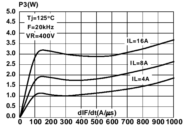
Fig 9 : Switching OFF losses versus dIF/dt
