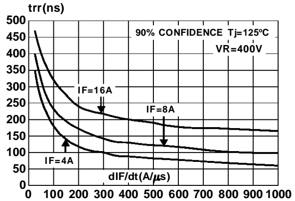
Fig 14 : Reverse recovery time versus dI_F/dt
